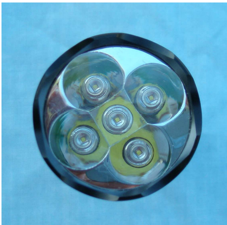
S-1300 flashlight head showing 5 Cree XRC LED's in a specialized spot/flood reflector housing.
